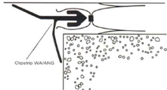
WALL - CORNER JOINT DETAIL
