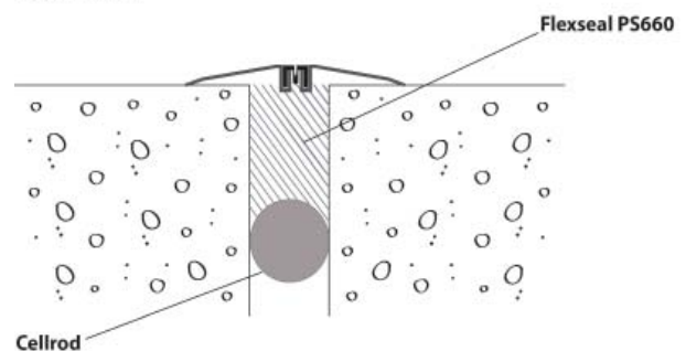
Floor Joint
