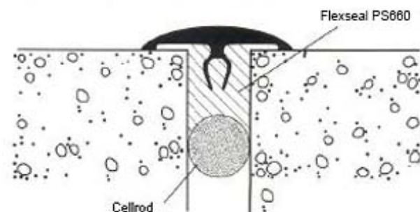
FLOOR - WATERTIGHT JOINT DETAIL
