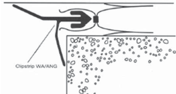
WALL - CORNER JOINT DETAIL
