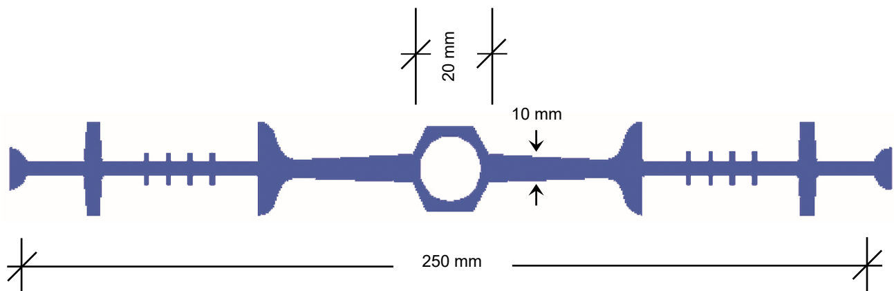
Center fix for expansion & construction joints (AB234)
