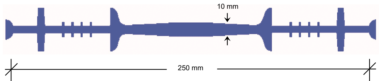
Center fix for expansion & construction joints (AB234)
