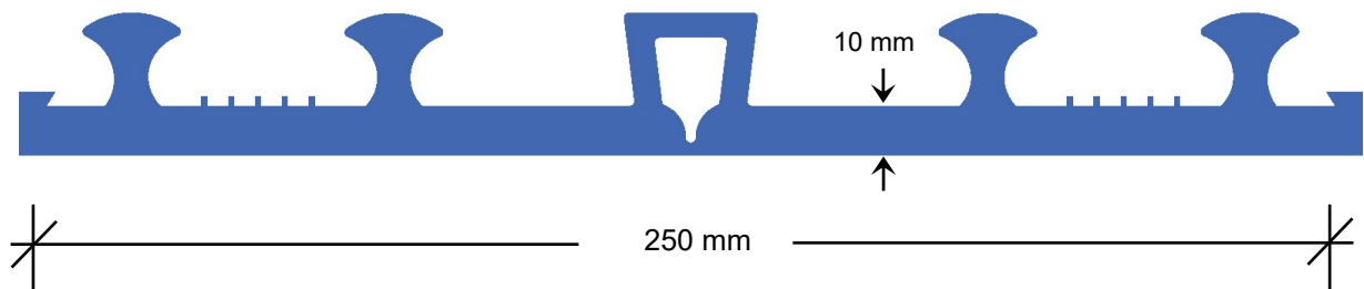
External fix for expansion & construction joints (AB232)
