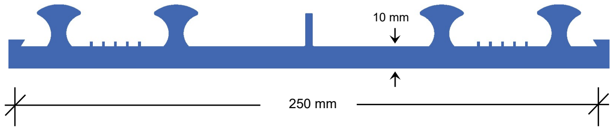
External fix for construction joints (AB231)
