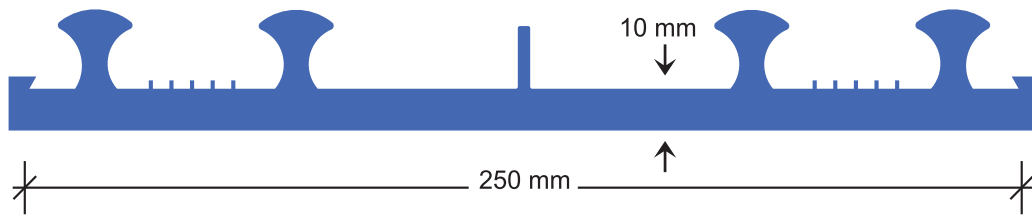
External fix for construction joints (AB231)
