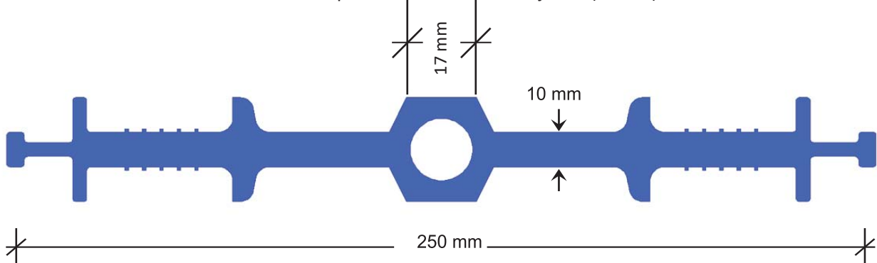
Center fix for expansion & construction joints (AB234)
