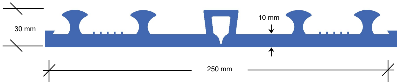
External fix for expansion & construction joints (AB232)
