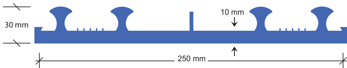
External fix for construction joints (HA231)
