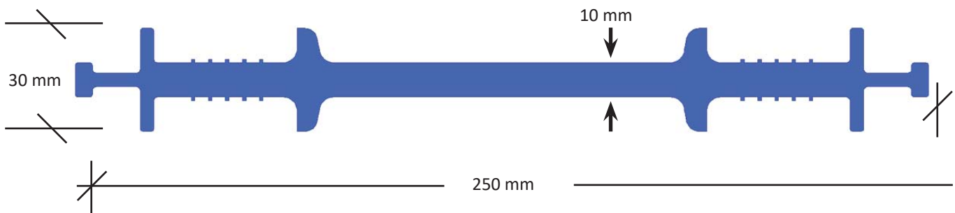
Center fix for construction joints (HA223/HA233)
