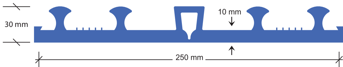
External fix for expansion & construction joints (HA232)
