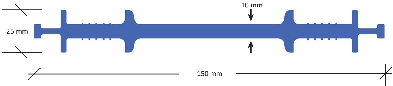
Center fix for construction joints (HA153)
