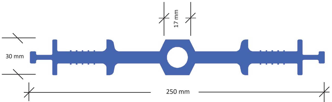
External fix for construction joints (HA231)
