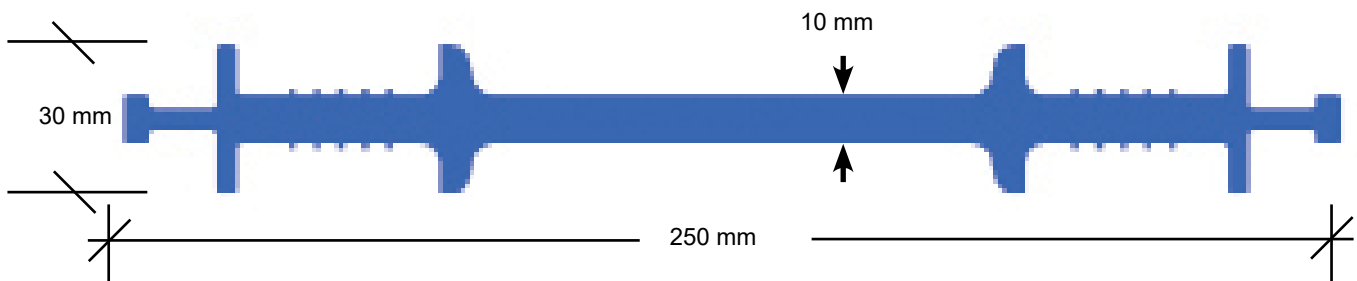
Center fix for construction joints (HA233)
