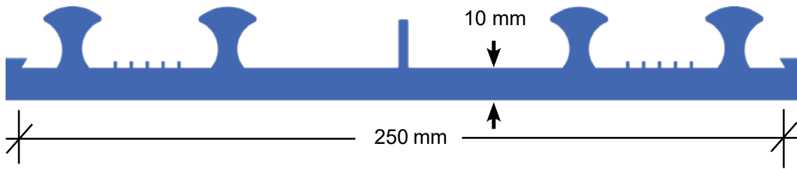
External fix for construction joints (HA231)
