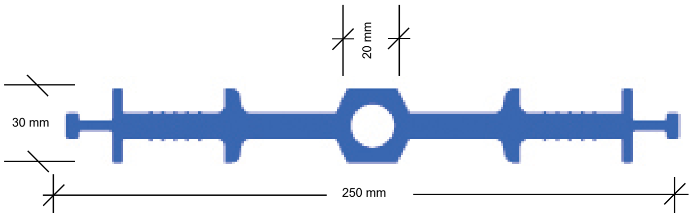
Center fix for expansion & construction joints (HA234)
